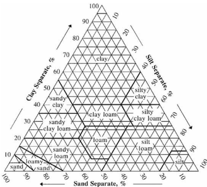
Figure 1. The soil textural triangle is used to categorize soils based on the proportion of sand, silt, and clay particles.
