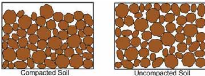
Figure 3. Soil compaction occurs, then soil particles are compressed, and the pore space between particles decreases.
